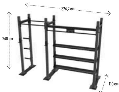
POWER RACK WITH SHELVES 1-1 SKU: 30-03101
